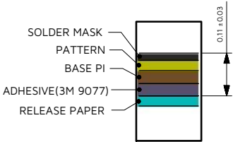
DETAIL B SCALE 80x FLEX LAYER
