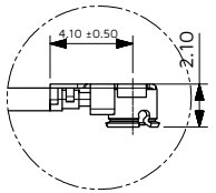
DETAIL A SCALE 5:1 CONNECTOR
